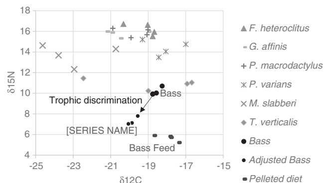
Fig. 4. Isotopic \delta^{15}N and \delta^{12}C signatures of the semi-extensively cultured bass, pelleted diet and likely prey items that enter the ponds. Adjusted D. labrax is the isotopic signature of the bass without the isotopic discrimination that occurs during assimilation of the diet into the consumer tissue.
